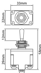
Double Pole
